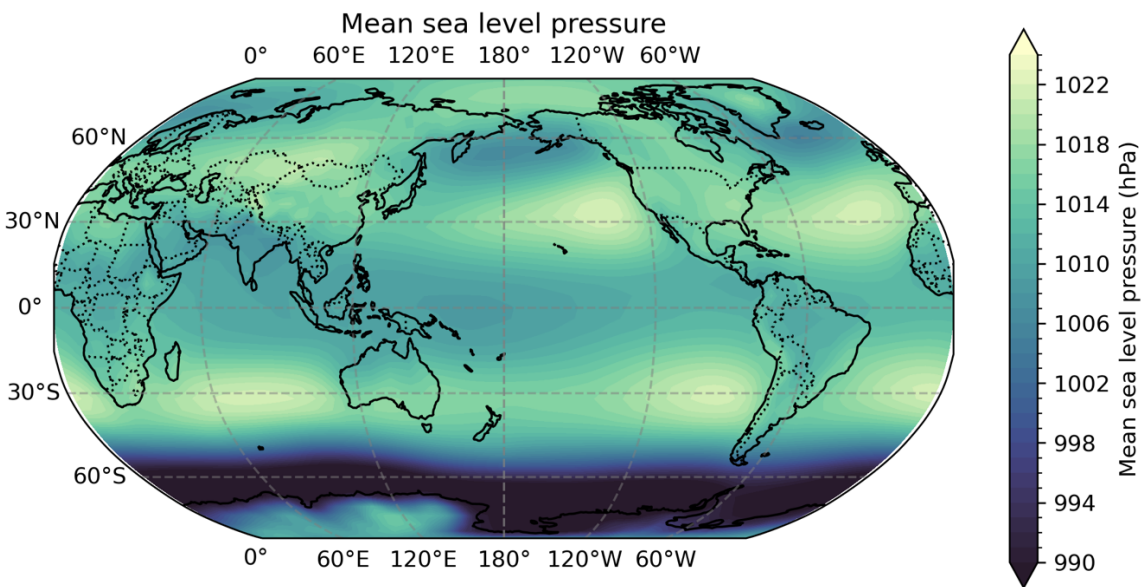
Figure 2. Annual mean sea-level pressure from July 2005 through June 2015 from the ERA5 reanalysis product. Figure generated by Professor Lawman using Python.
