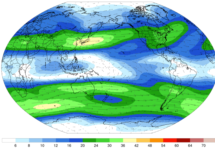
Figure 3. Annual mean 250 hPa wind speed (units: m/s) from the ERA5 atmospheric reanalysis product (2005-2015). Figure generated using the Climate Reanalyzer ( https://climatereanalyzer.org/research_tools/monthly_maps/ ).
