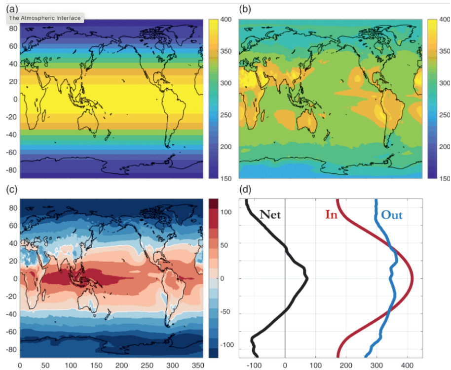
Figure 1. Long-term mean energy fluxes at the top of the atmosphere (TOA) averaged from July 2005 through June 2015 ( \text{W/m}^2 ). (a) Incoming shortwave radiation. (b) Outgoing radiation (reflected solar and longwave). (c) Net radiation (incoming - outgoing). (d). Zonal means of incoming, outgoing and net radiation. Figure credit: Kris Karnauskas
