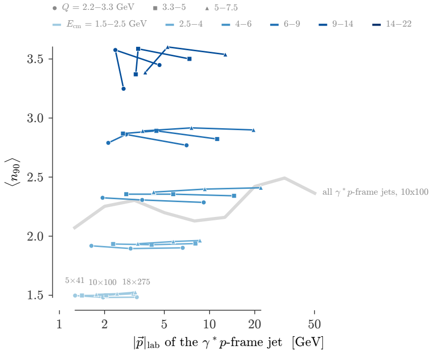
Jets clustered in the colour rest frame with n_{90} computed from their lab momenta, in cells of fixed jet energy in that frame and fixed Q , across the three beam configurations: median slope +0.00 , against +0.03 for the inclusive curve (grey).
