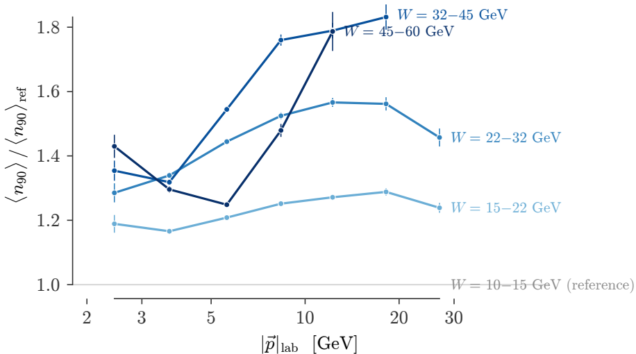
Fractional frame-dependent fragmentation shift at the EIC: the ratio of \langle n_{90} \rangle at fixed lab momentum between W slices.
