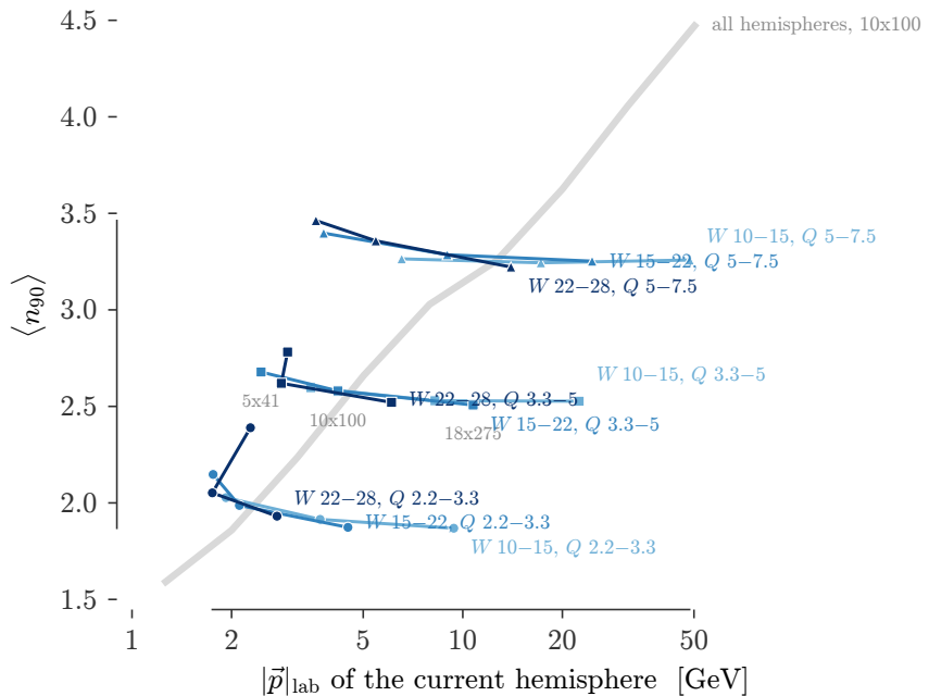
Each line is one cell of fixed (W, Q) , so fixed colour-frame kinematics, measured in three EIC beam configurations. The beam energy changes only the lab frame. Along each line the current hemisphere's lab momentum moves by up to a factor of ten and \langle n_{90} \rangle does not follow: median slope d \ln \langle n_{90} \rangle / d \ln p = -0.05 per cell, against +0.28 for the inclusive curve (grey). Marker shape encodes the Q bin.
