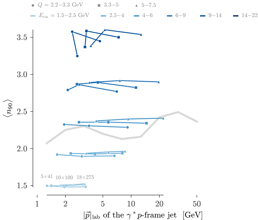
Jets clustered in the colour rest frame with n_{90} computed from their lab momenta, in cells of fixed jet energy in that frame and fixed Q , across the three beam configurations: median slope +0.00 , against +0.03 for the inclusive curve (grey).
