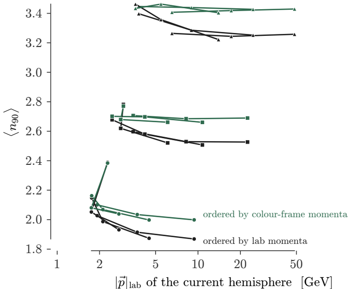
The same hemispheres in fixed (W, Q) cells across the three beam configurations, with n_{90} built from lab momenta (dark) and from colour-frame momenta (green). The particles are identical; only the frame in which they are ordered differs. Ordering in the lab leaves a residual slope of -0.050 because a large boost pushes the ordering towards light-cone momentum and concentrates the jet in fewer particles; ordering in the colour frame leaves -0.008 .
