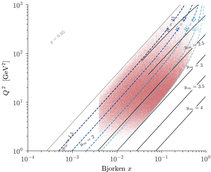
Solid: rapidity of the colour rest frame ( \gamma^* p CM) relative to the lab, y_{\text{cm}} ; a jet at fixed lab momentum is seen in that frame with momentum reduced by roughly e^{-y_{\text{cm}}} along the axis. Dashed: lines of constant W . Red: the selected current jets.
