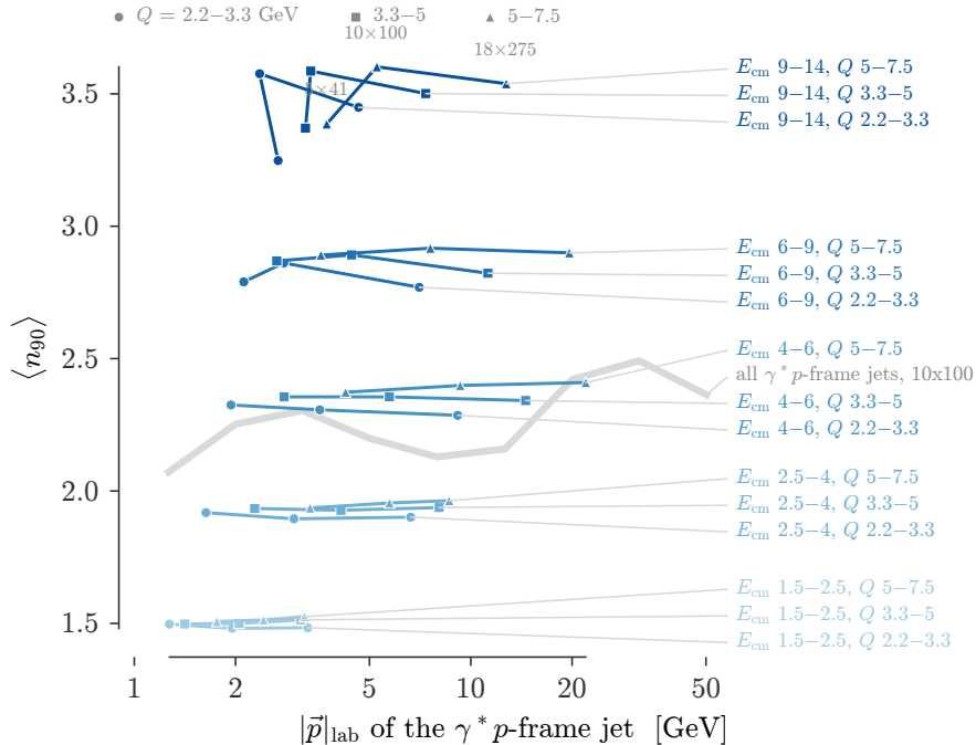
Jets clustered in the colour rest frame with n_{90} computed from their lab momenta, in cells of fixed jet energy in that frame and fixed Q , across the three beam configurations: median slope +0.00, against +0.03 for the inclusive curve (grey).
