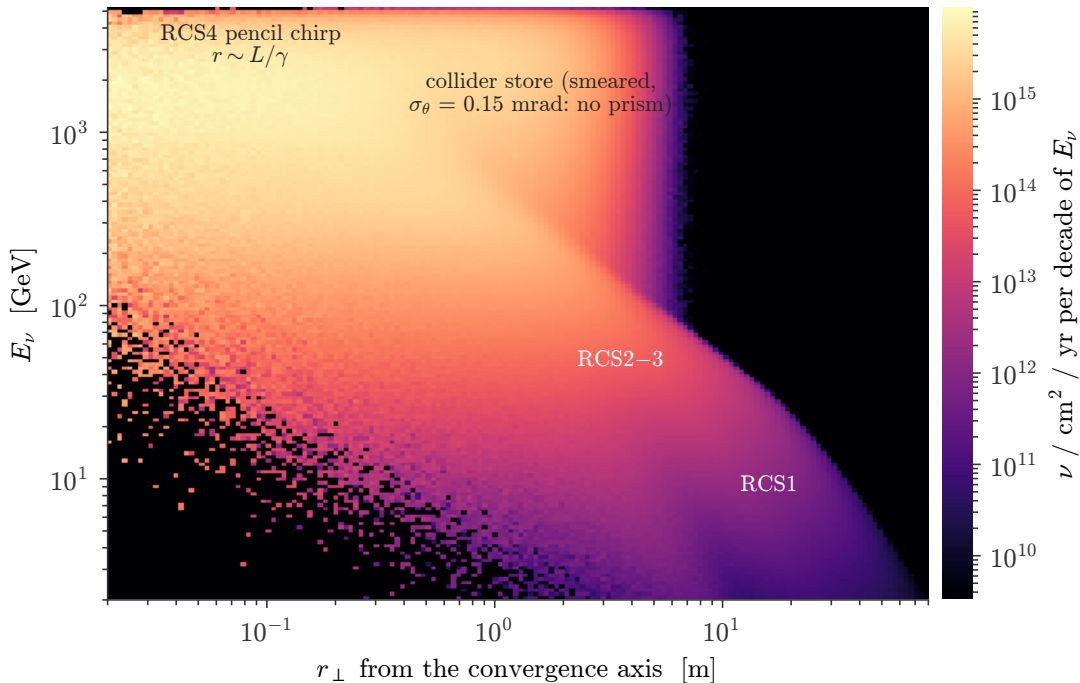
Fluence at the convergence hall (9.25 km): every stage on one axis
