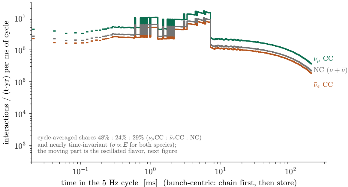
Flavor composition vs time at the deep hall (9.25 km): shares barely move
