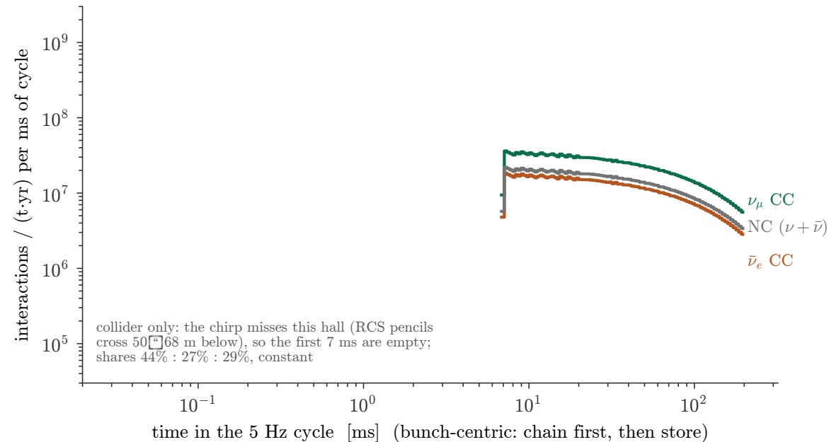
Flavor composition vs time at the near hall (1.3 km): silent until the store
