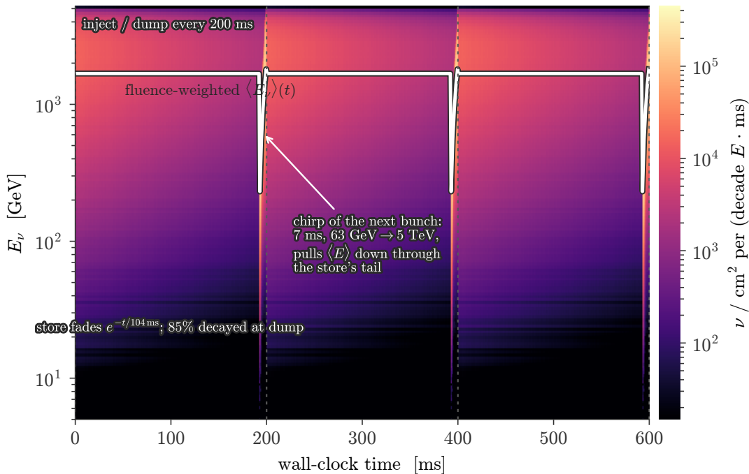
Three 5 Hz cycles, wall-clock: sawtooth store, chirp in the overlap window
