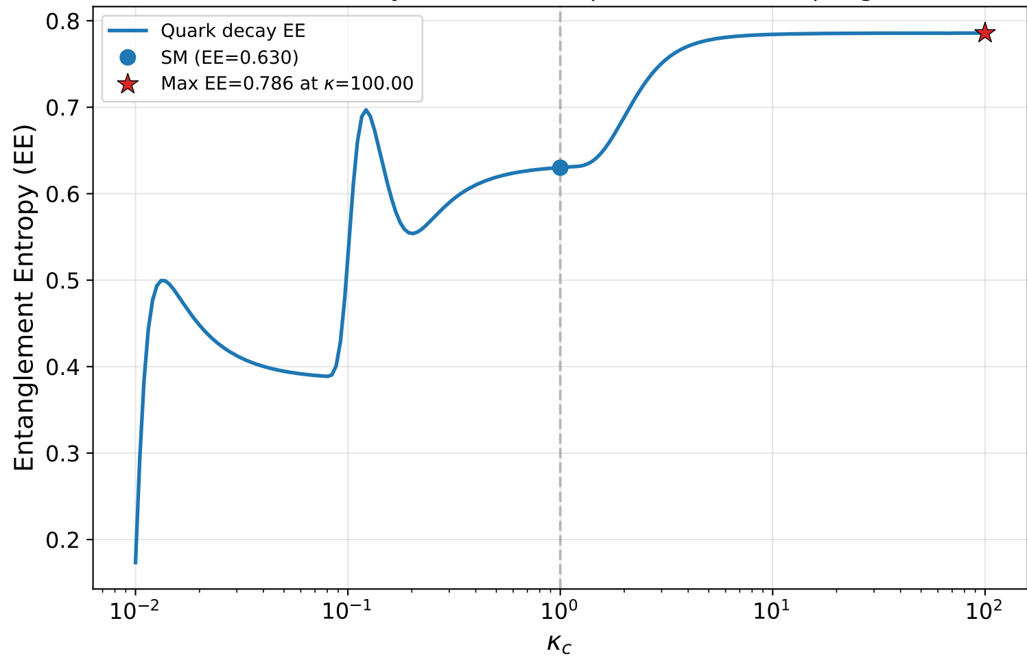
Weak-Decay EE vs charm quark Yukawa coupling
