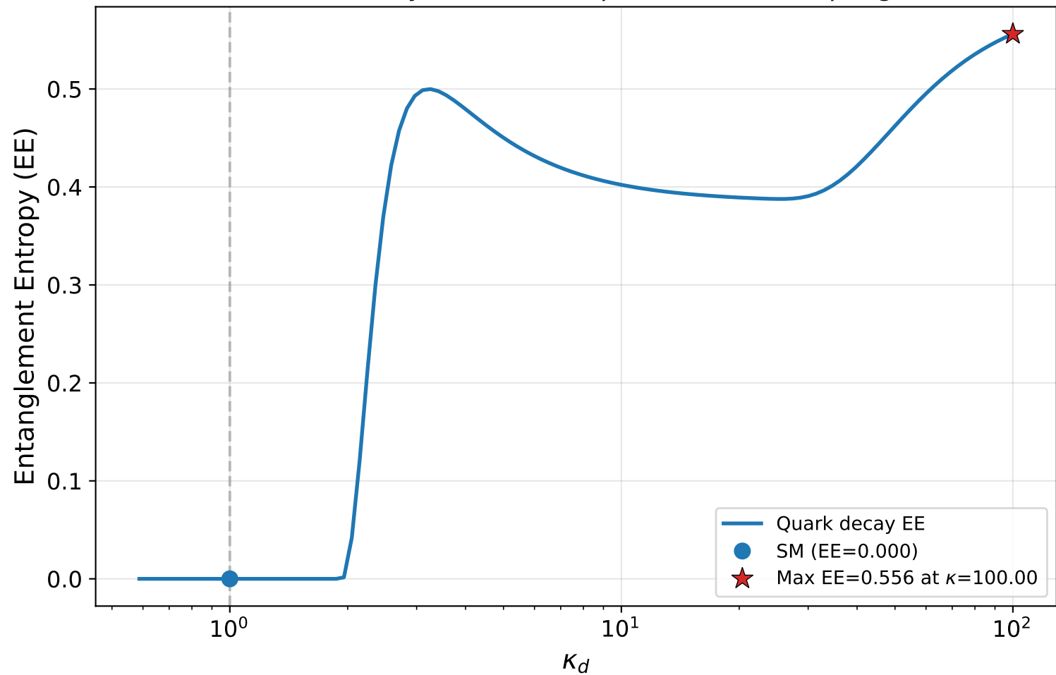
Weak-Decay EE vs down quark Yukawa coupling
