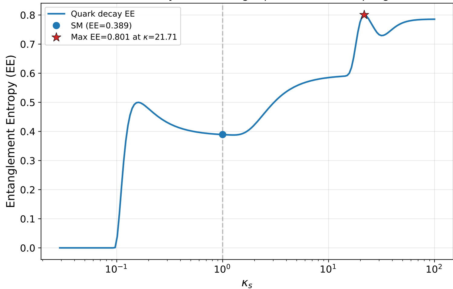
Weak-Decay EE vs strange quark Yukawa coupling
