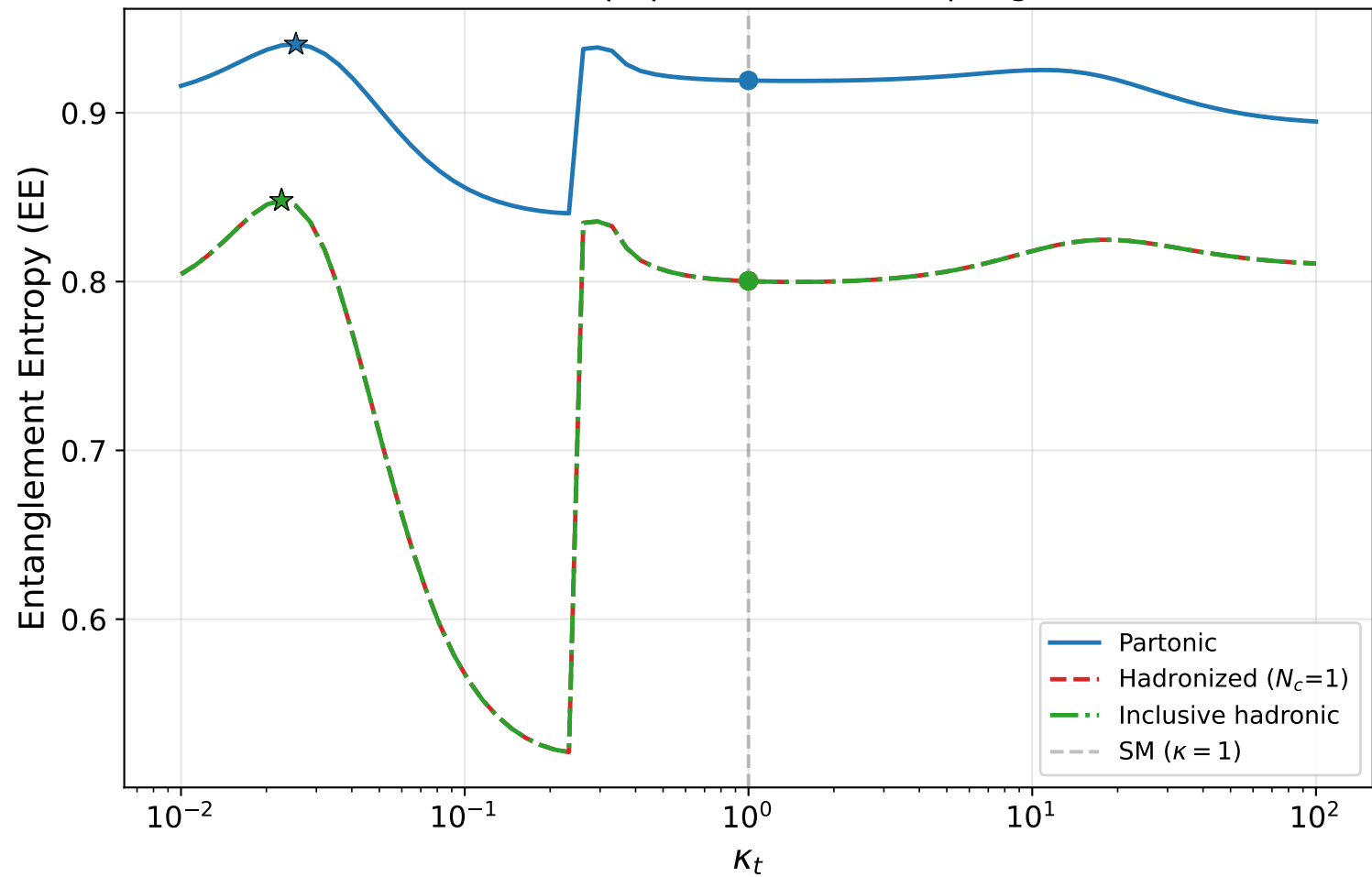
EE vs top quark Yukawa coupling
