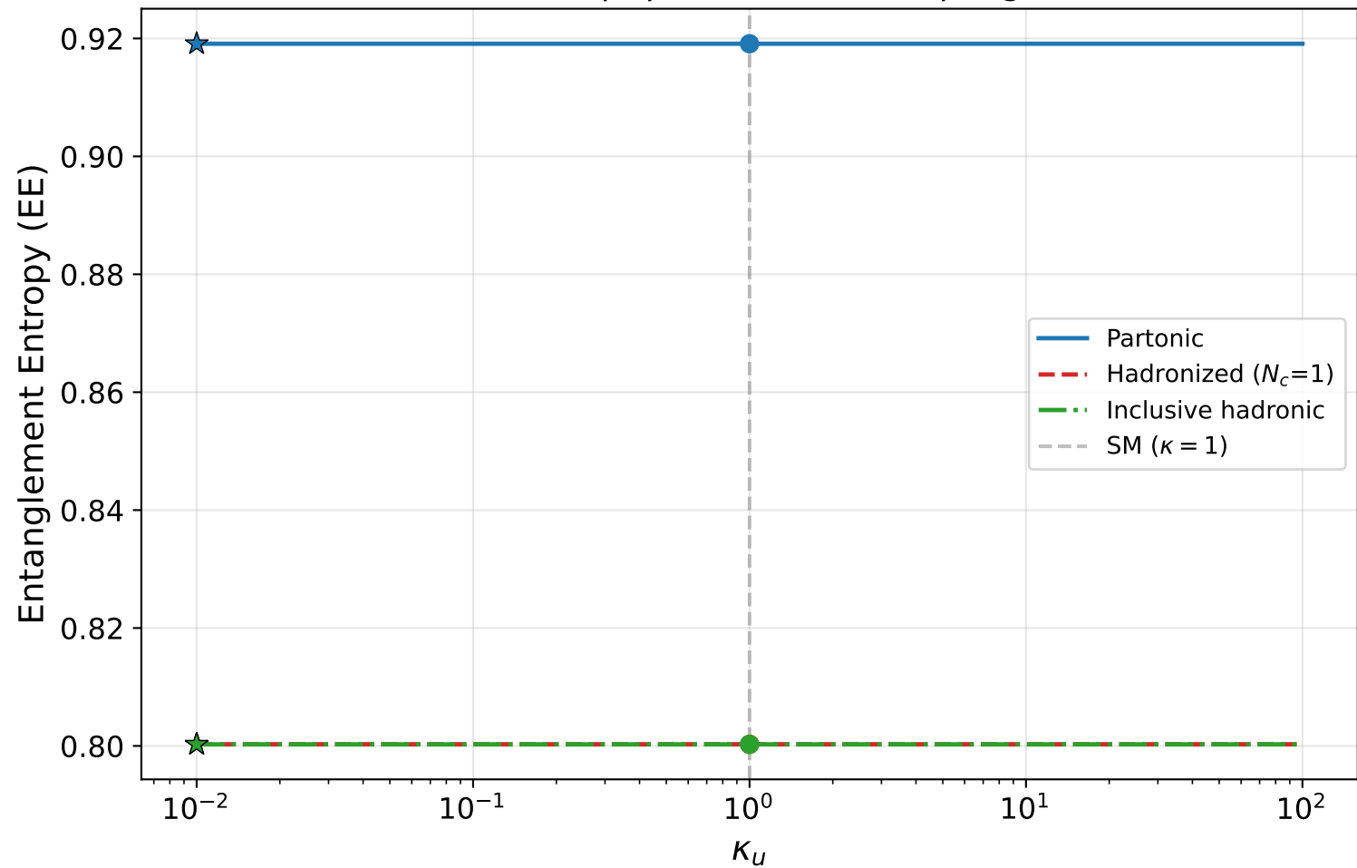
EE vs up quark Yukawa coupling
