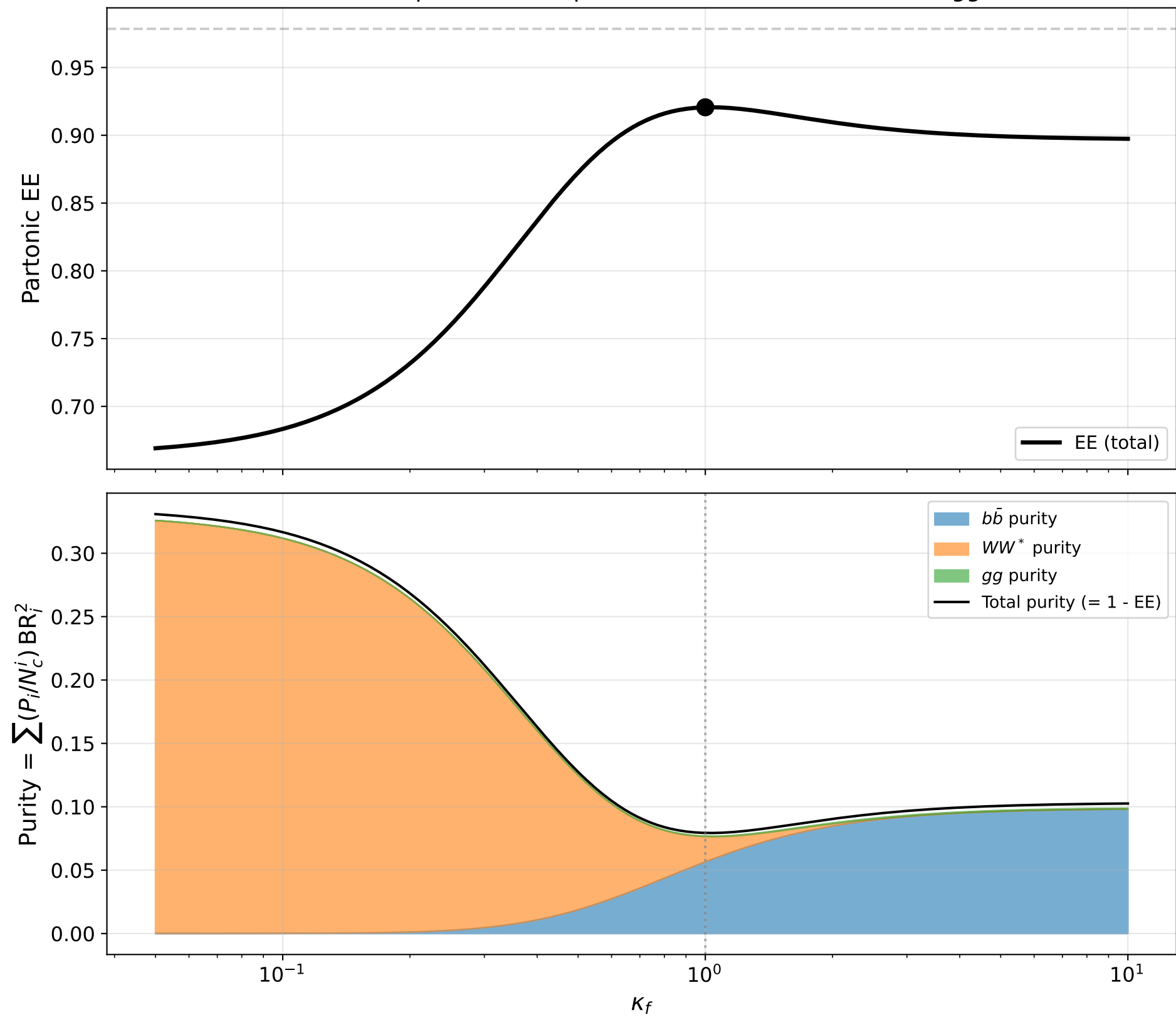
EE decomposition: competition between b\bar{b} , WW^* , and gg
