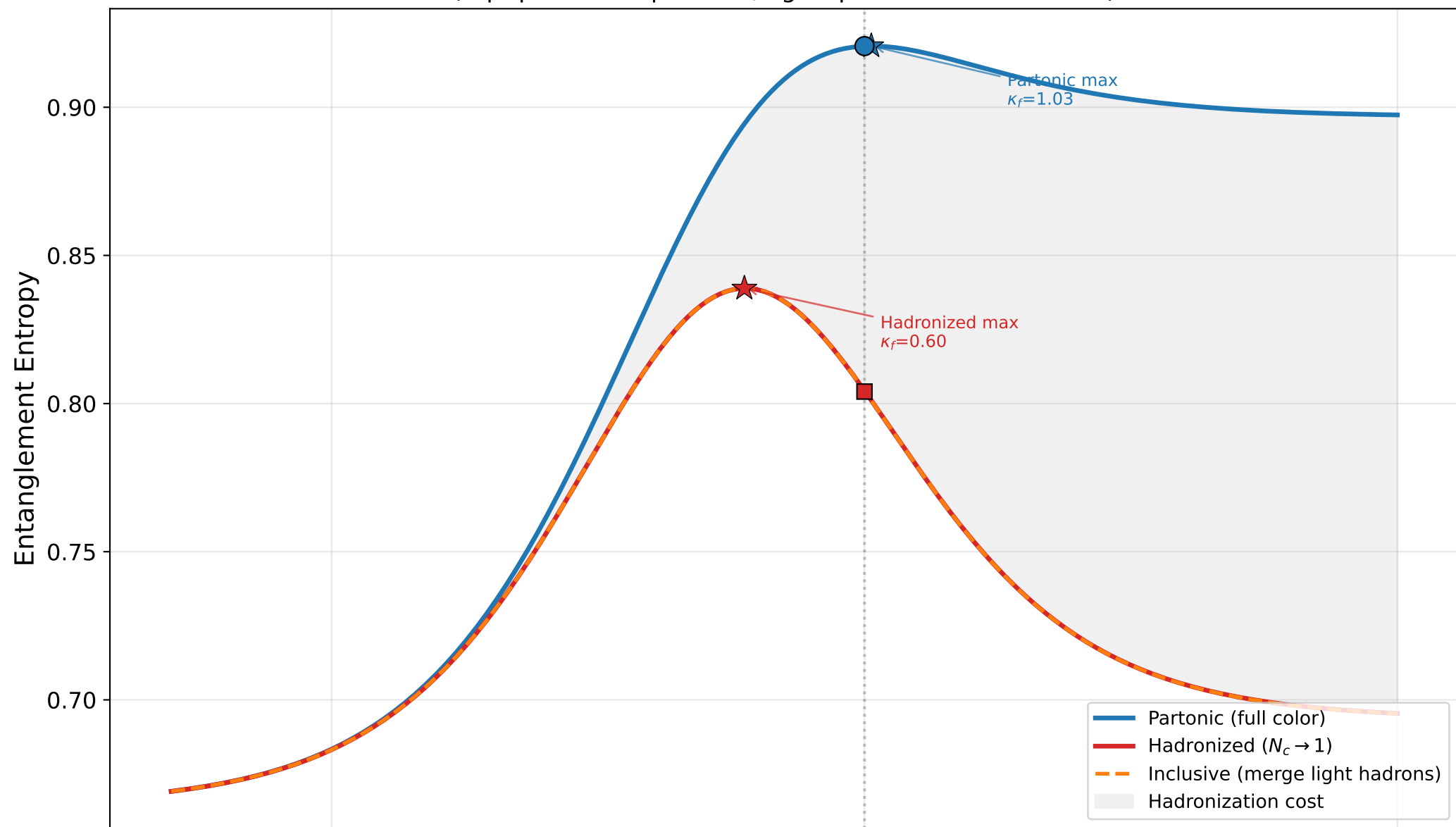
Higgs EE: partonic vs hadronized regimes (top quark sees partonic; light quarks see hadronized)
