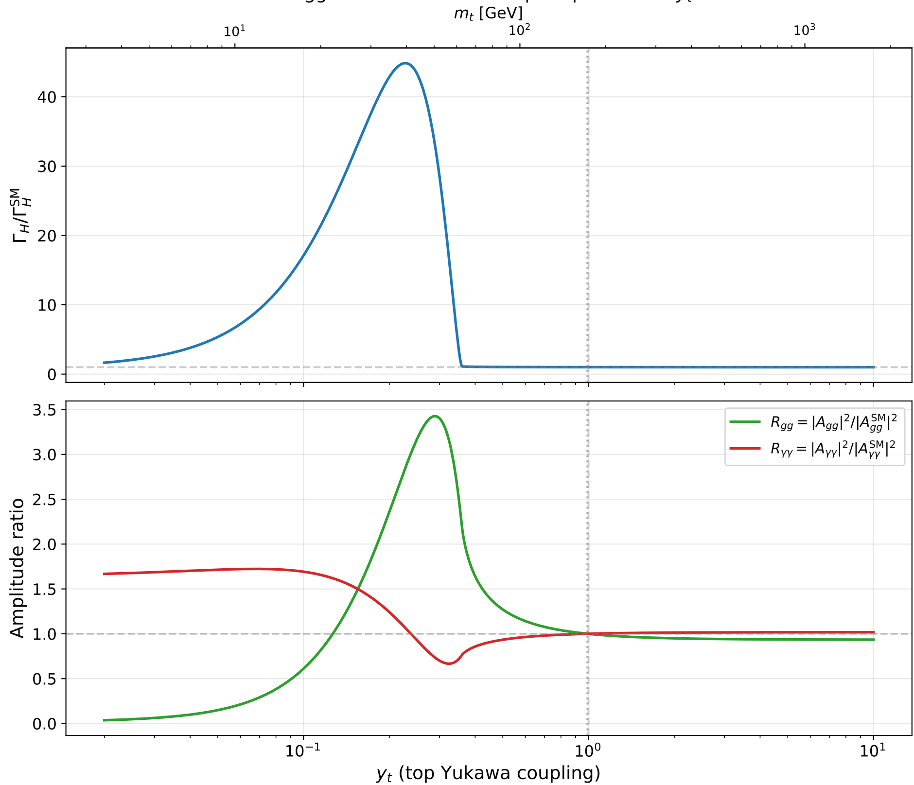
Higgs Total Width and Loop Amplitudes vs y_t
