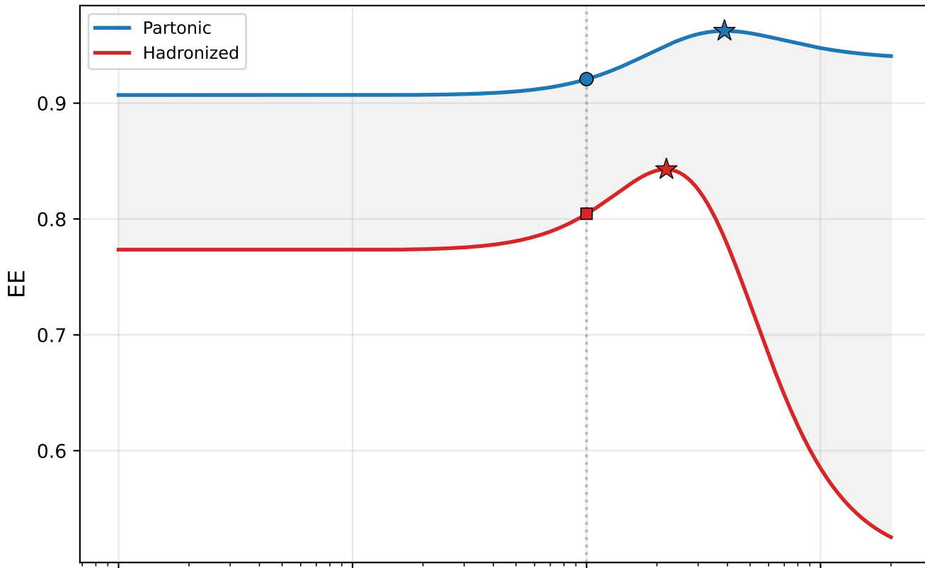
charm ( \kappa_c ): part. max @ 4.11, hadr. max @ 3.74
