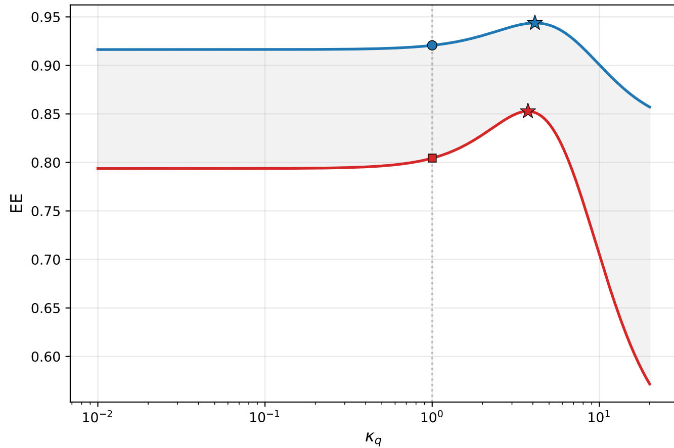
charm ( \kappa_c ): part. max @ 4.11, hadr. max @ 3.74
