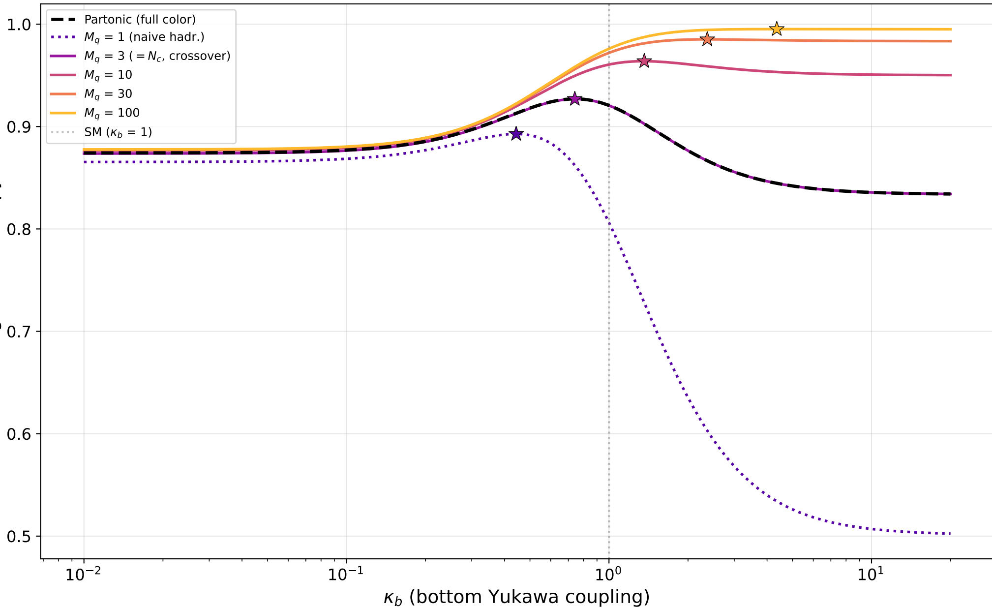
Higgs EE vs \kappa_b at different hadronic multiplicities
