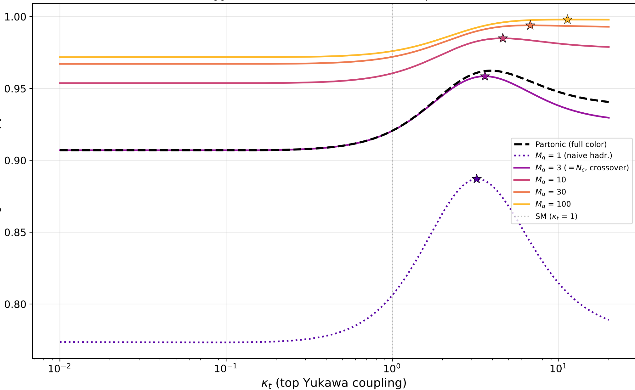
Higgs EE vs \kappa_t at different hadronic multiplicities
