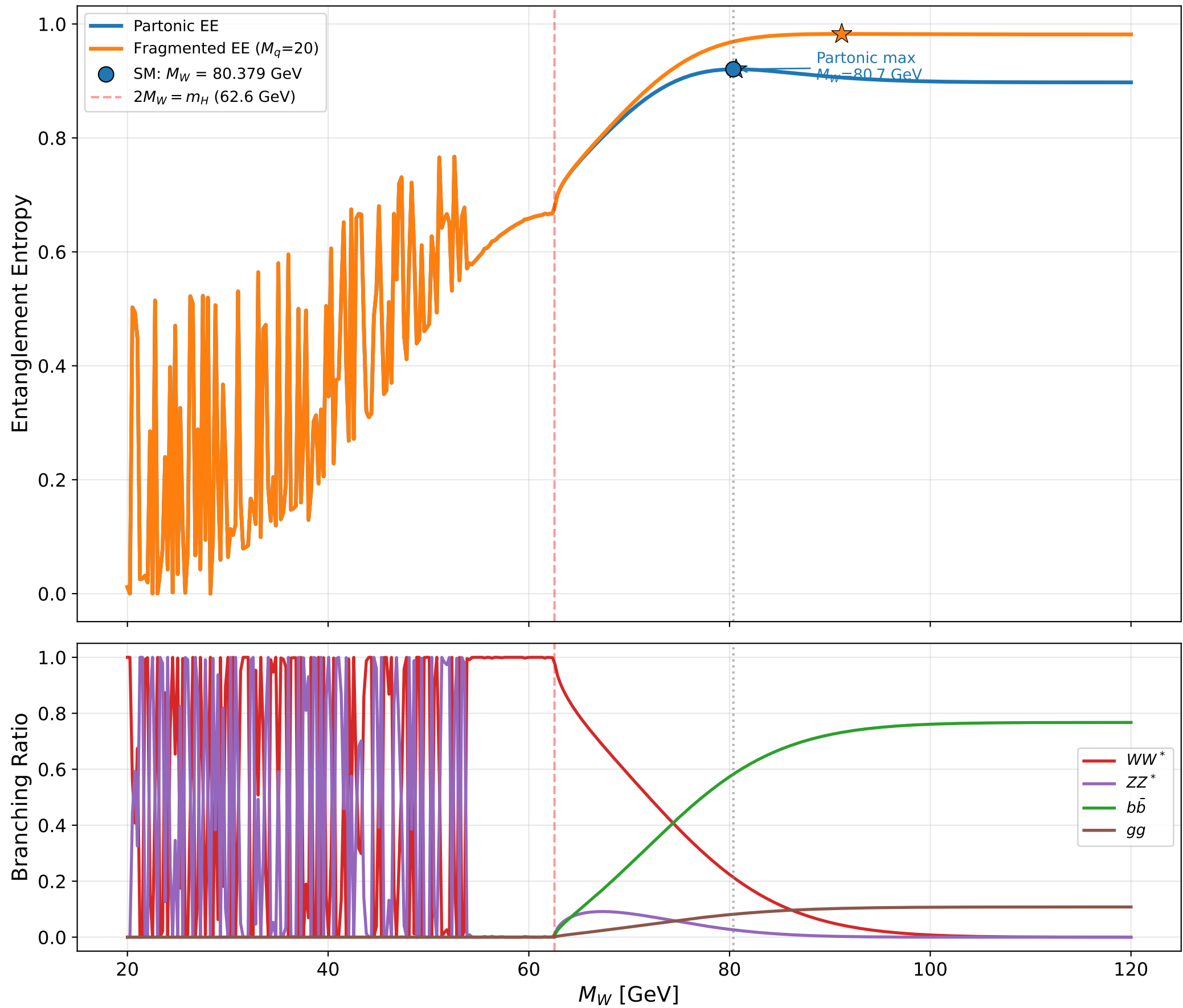
Higgs decay EE vs M_W (SM W mass is near the EE maximum)
