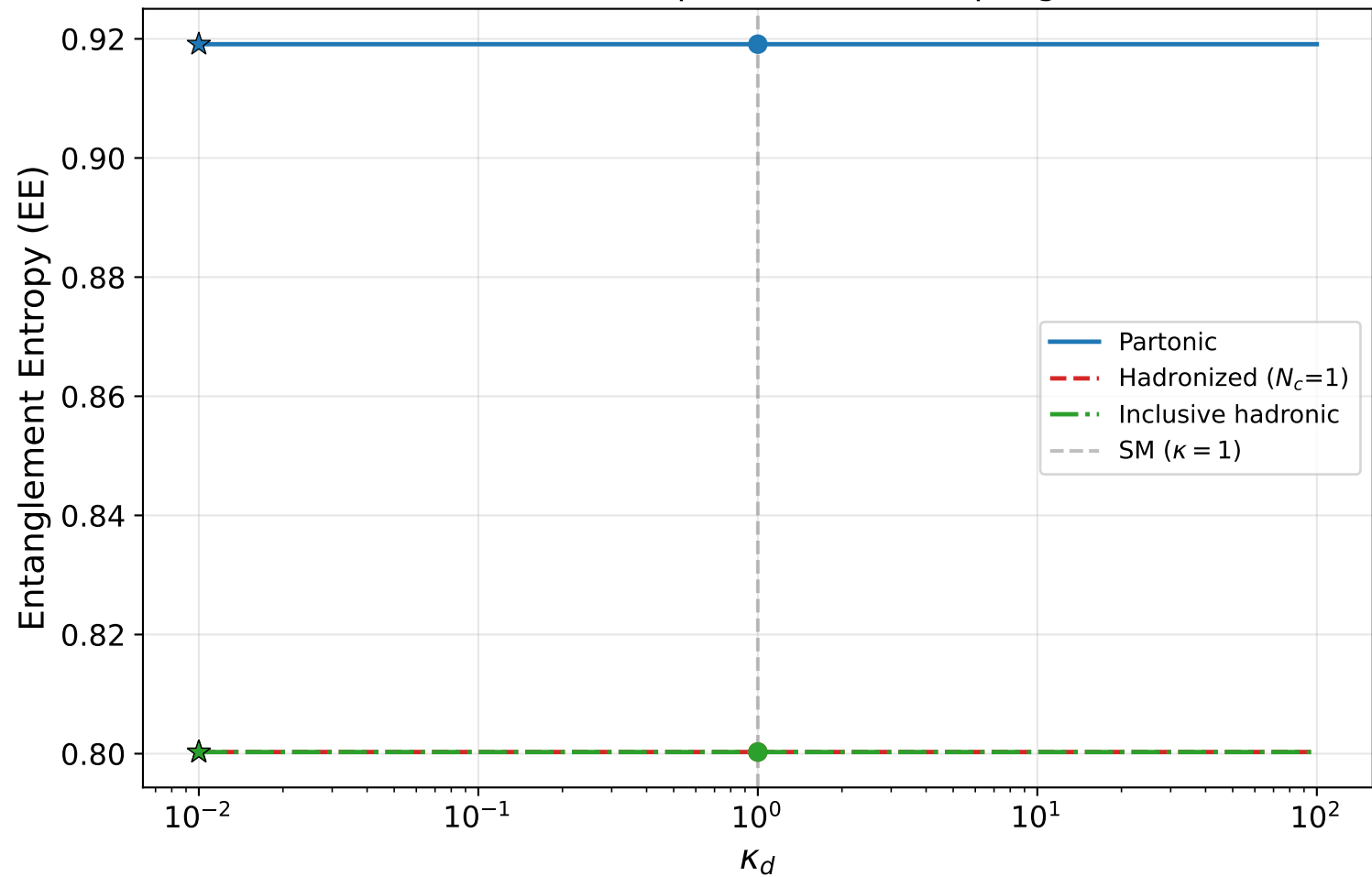
EE vs down quark Yukawa coupling
