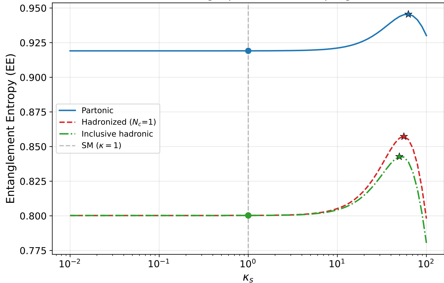
EE vs strange quark Yukawa coupling
