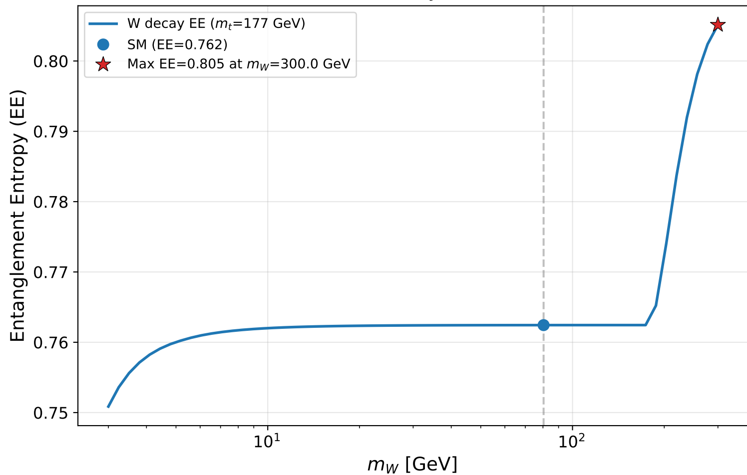
W Boson Decay EE vs m_W
