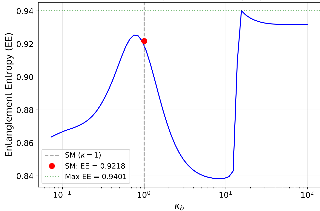
EE vs bottom quark Yukawa coupling
