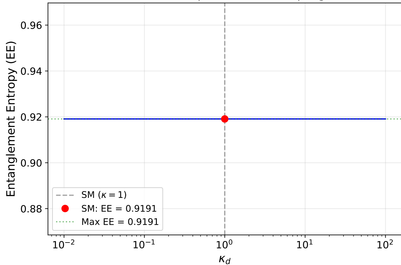
EE vs down quark Yukawa coupling
