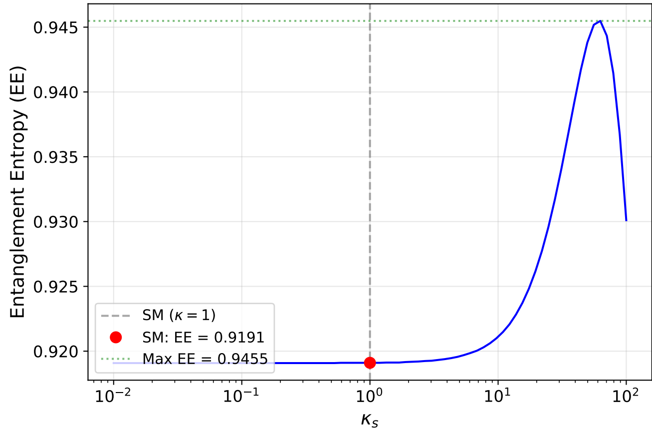
EE vs strange quark Yukawa coupling
