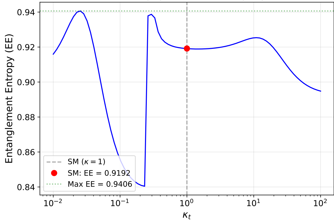
EE vs top quark Yukawa coupling
