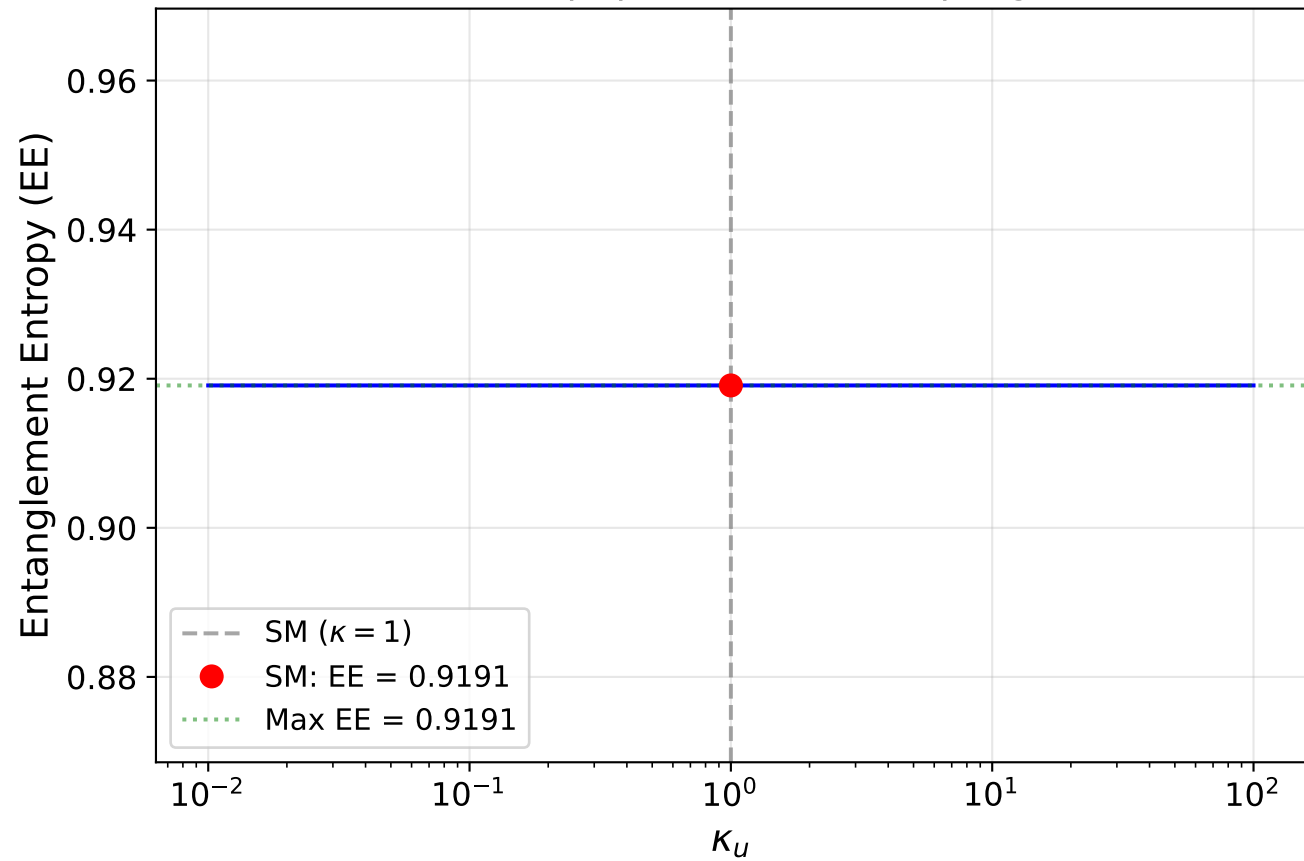
EE vs up quark Yukawa coupling
