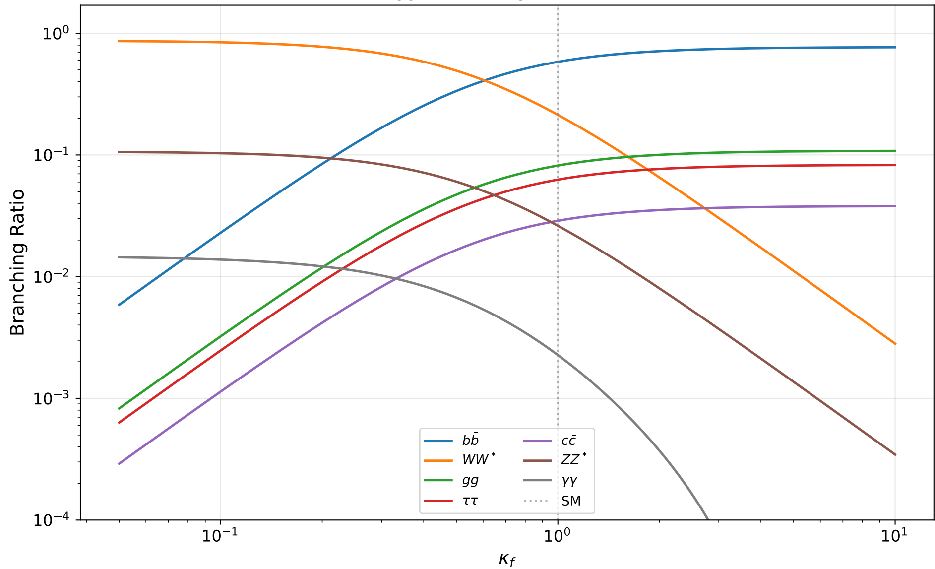
Higgs Branching Ratios vs K_f
