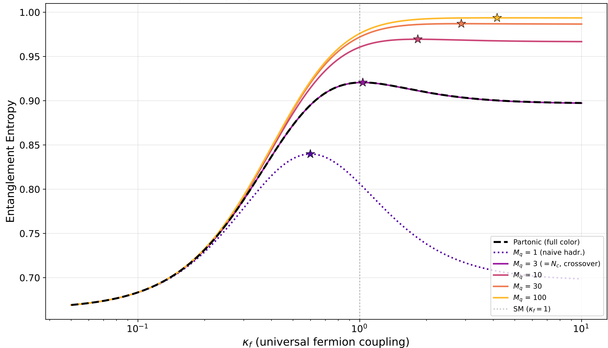
Higgs EE vs \kappa_f at different hadronic multiplicities Higher multiplicity \rightarrow hadronization increases EE \rightarrow optimum shifts
