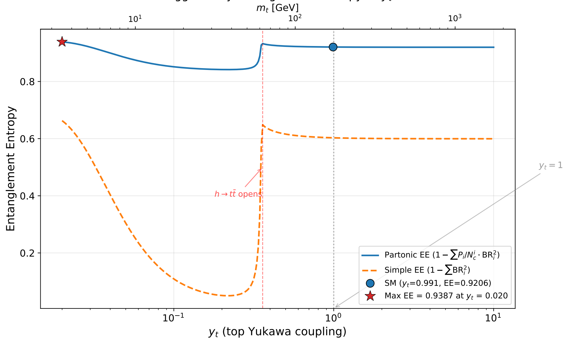
Higgs Decay Entanglement Entropy vs y_t
