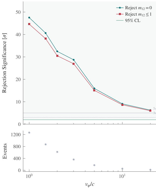
FIG. 3. Rejection significance for the finite-speed signal hypothesis as a function of the assumed signal speed v_\psi/c . Blue circles: rejection of m_{12} = 0 (no correlation); red squares: rejection of m_{12} \leq 1 (locality). Horizontal lines mark 95% CL (1.96 \sigma ), 3 \sigma , and 5 \sigma thresholds. Bottom: number of events with v_{\text{signal}} > v_\psi .
