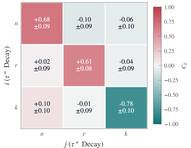
FIG. 1. Reconstructed spin correlation matrix C_{ij} in the \{n, r, k\} basis from 999 fully reconstructed \pi/\rho tau pairs, using polarimeter vectors. Entries show the central value \pm bootstrap uncertainty. The exact SM prediction, Eq. (2), is C = \text{diag}(+1, +1, -1) for any \beta ; deviations from unit magnitude reflect channel-dependent reconstruction dilution (see text).
