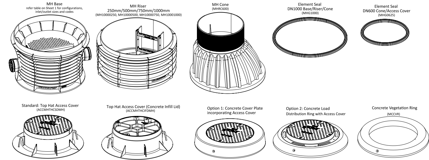
Figure 3 – Typical System Components
