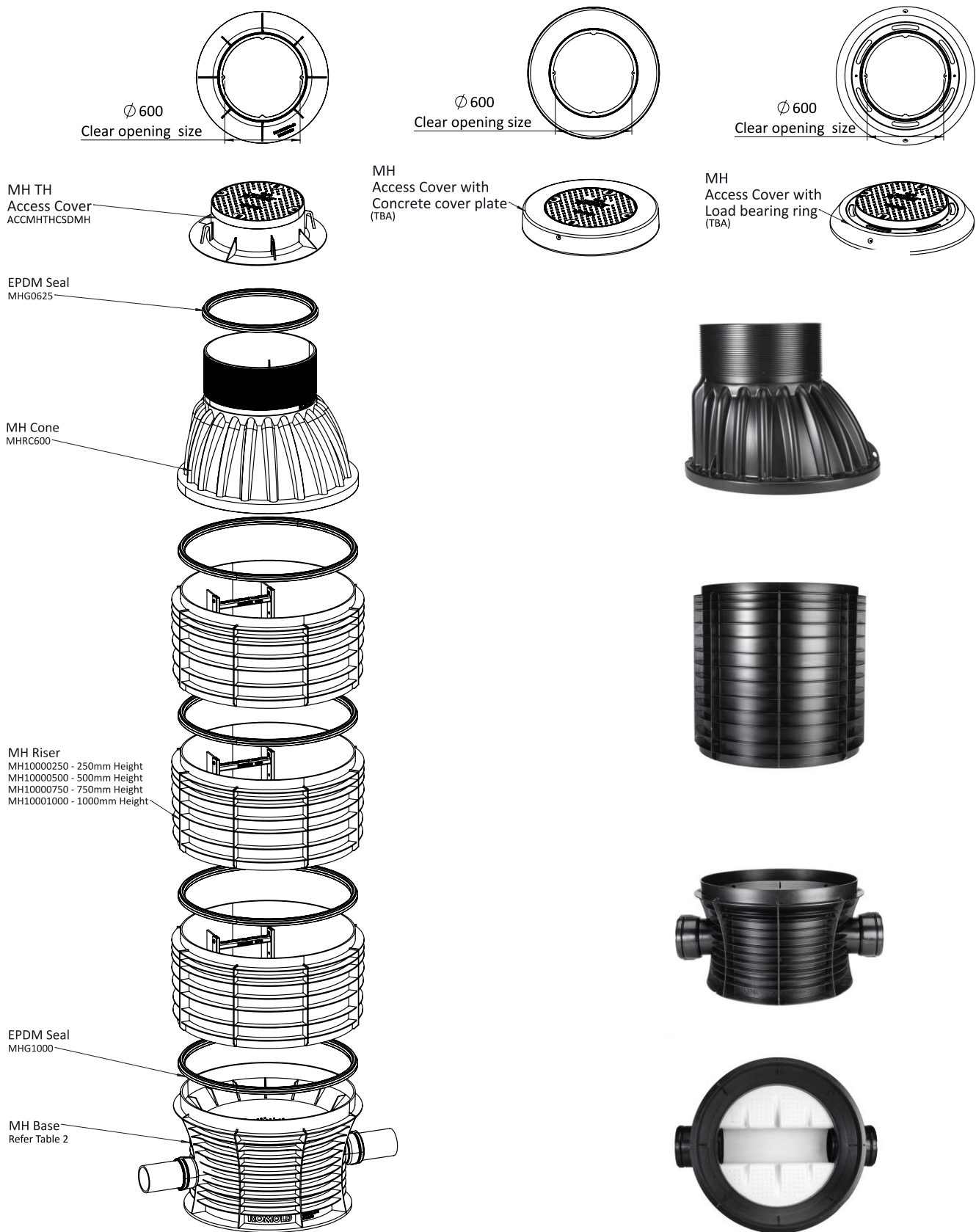
Figure 2 – Typical Installation options
