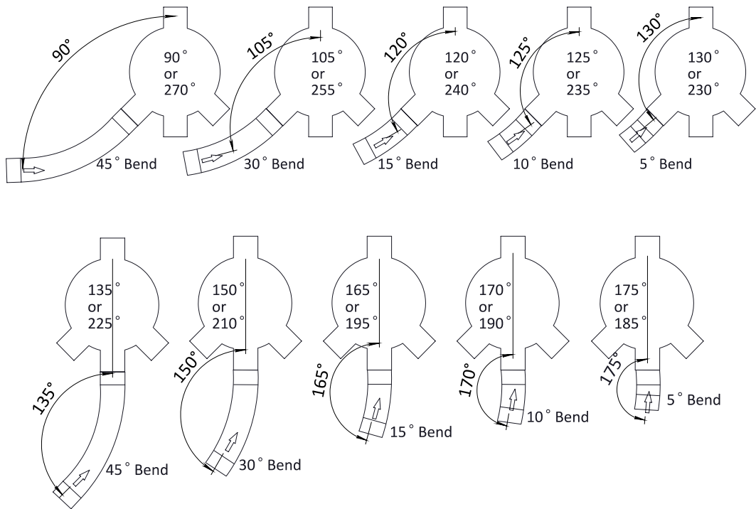
Figure 4 – Angles achieved using long radius bends
