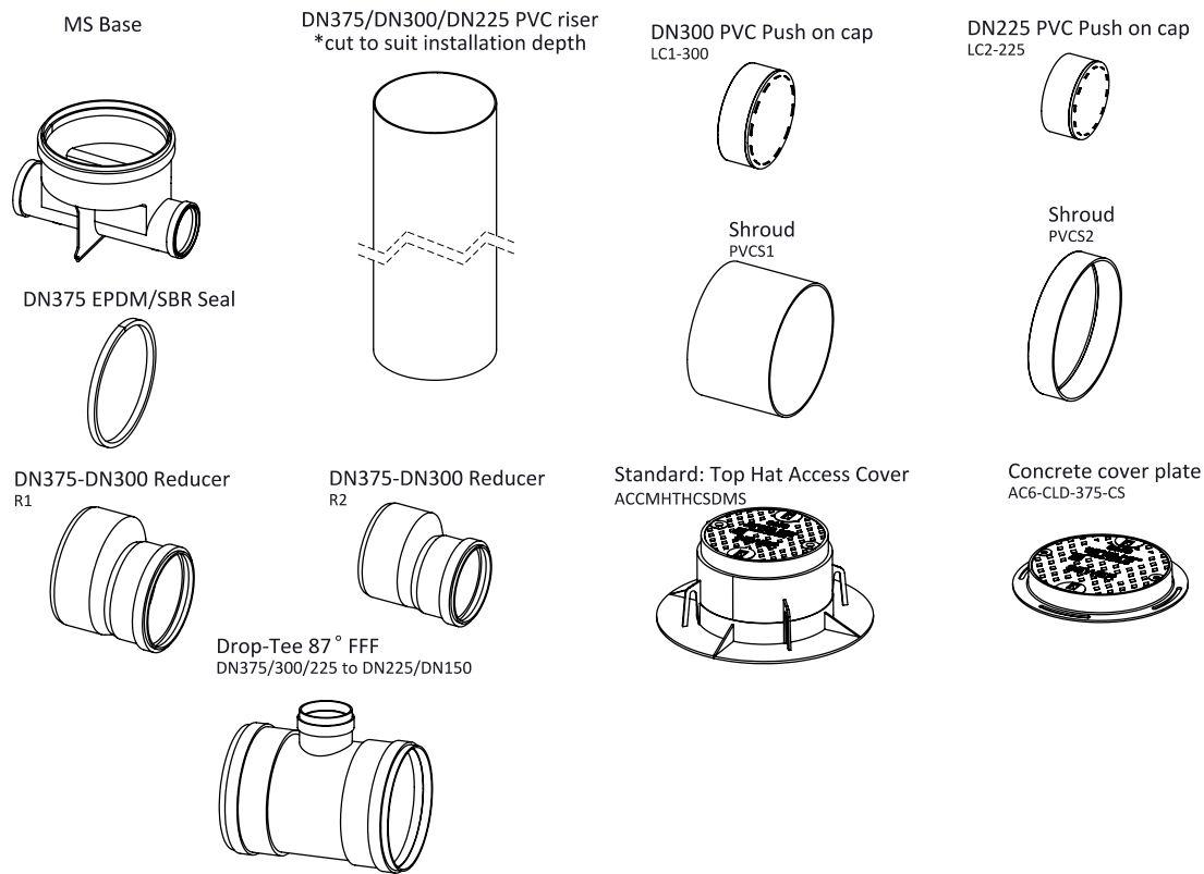
Figure 3 – Typical System Components
