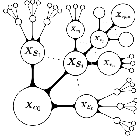
Figure 4: A tree decomposition (\mathcal{X}, F) of the overall conflict graph constructed from the instance of 1 \mid k_j, \text{rep} \mid \min_j \sum_i Z_{i,j} . Observe that the width of this decomposition is |X_v| - 1 = 4 .
