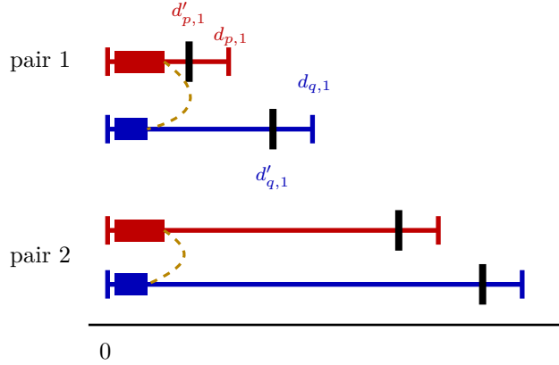
Figure 3: A connected pending pair: at least one of the two jobs must meet its early deadline.
