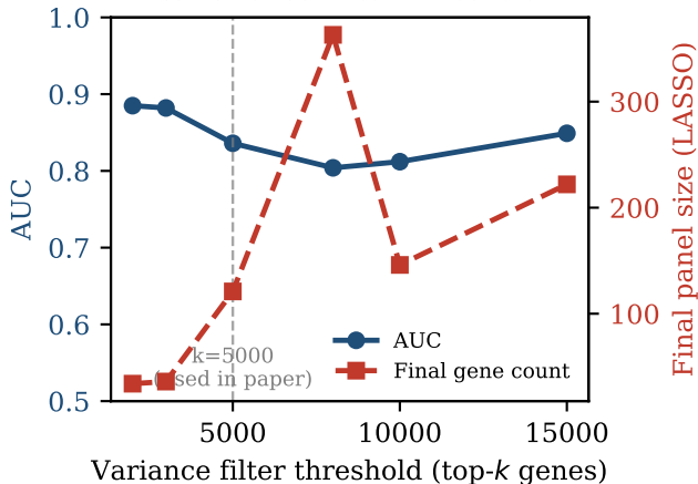
Sensitivity of Classification Performance to Variance Filter Threshold
