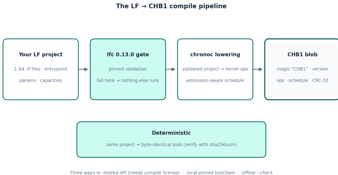
Compile pipeline
