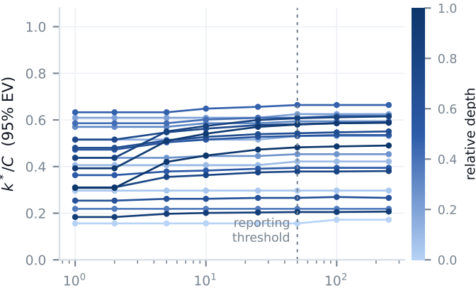
resnet18
