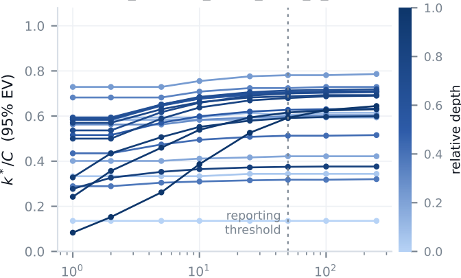
timm_convnext_tiny.fb_in22k_ft_in1k
