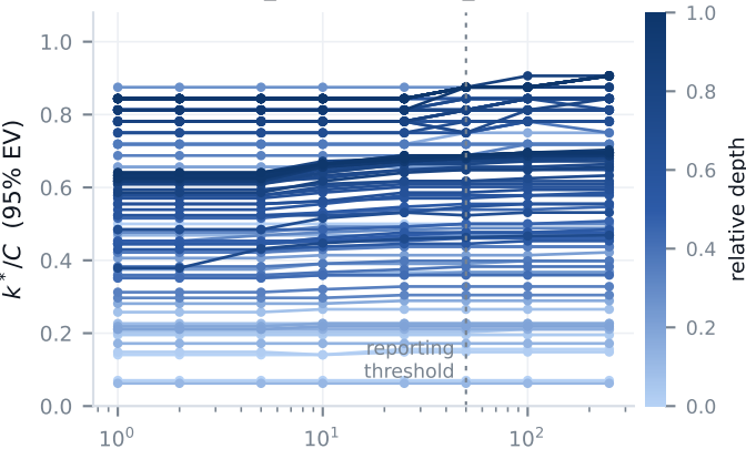
timm_densenet121.tv_in1k
