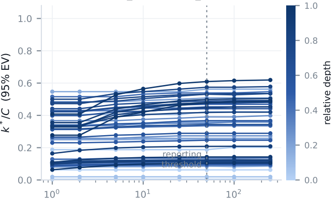
timm_resnet50.a3_in1k
