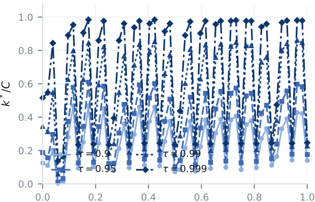
timm_resnet50.fb_ssl_yfcc100m_ft_in1k
