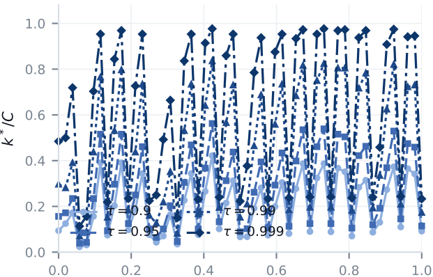
timm_resnet50.tv_in1k
