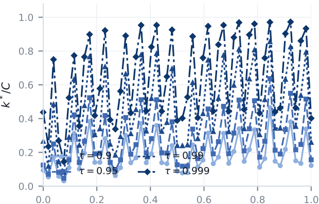
timm_resnext50_32x4d.tv_in1k
